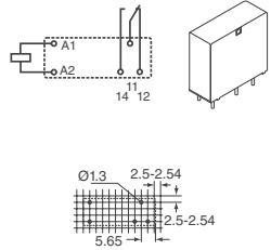
Fig. 5 — PCH Series
