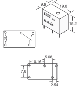
Fig. 6 — PCJ Series
