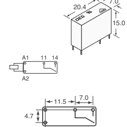
Fig. 6 — PCJ Series
