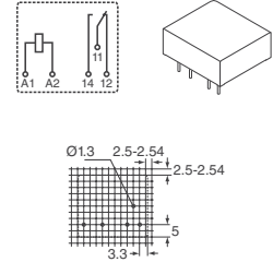
Fig. 4 — Relay Card E - Vertical
