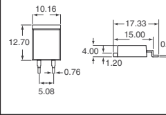
Fig. 1 — FPS2-T220 (Surface Mount)
