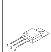
Fig. 8 — TO-220AB
