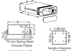
Fig. 4 - Plastic Instrument Cases - 1598 Series
